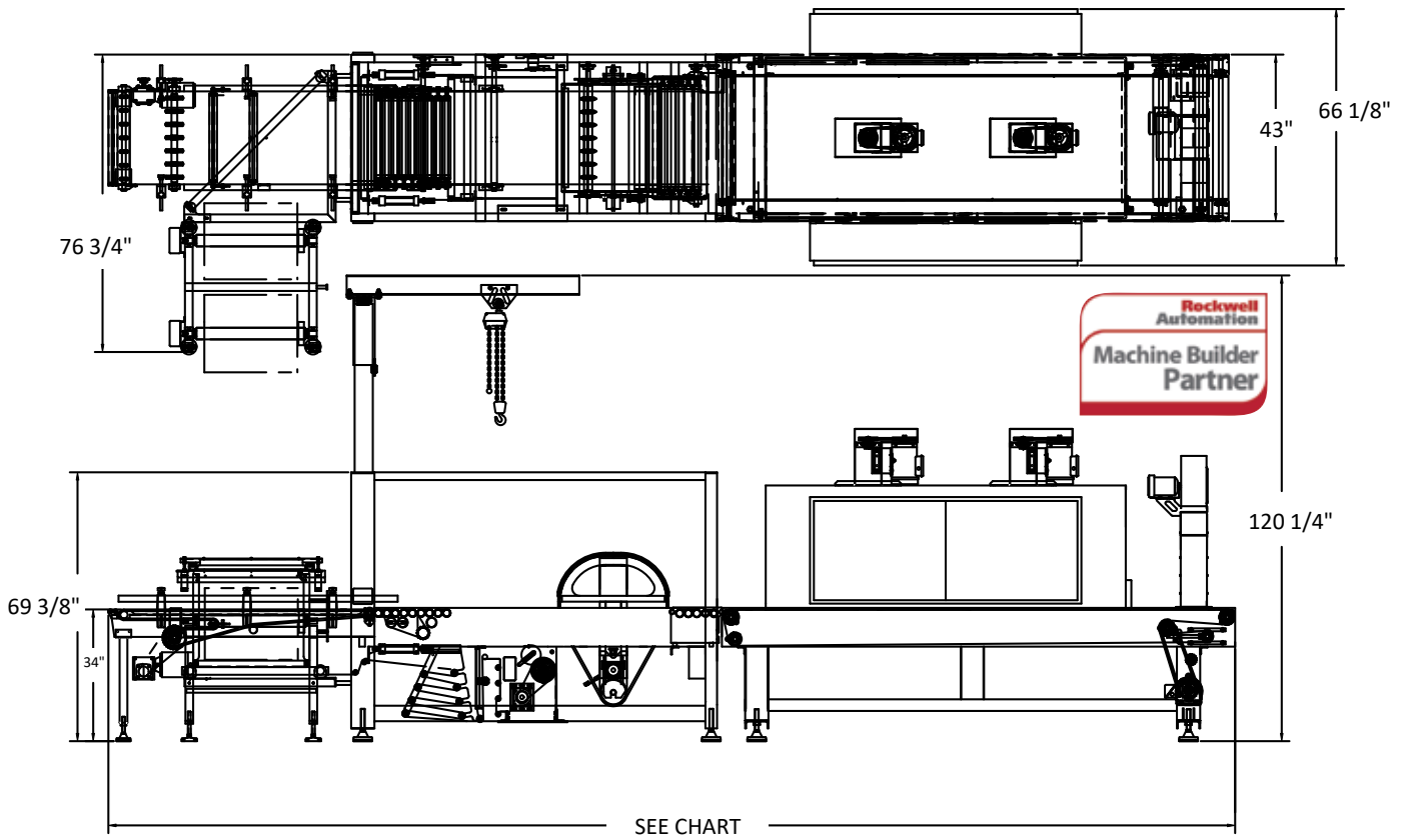
Left hand BPTW-5301 with dual zone tunnel, final layout may vary. Opposite hand available on request.
